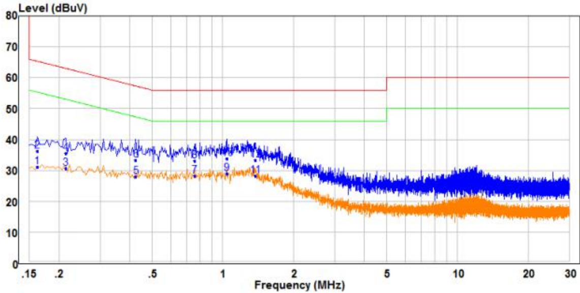
Trace: 1 Condition: EN55015-QP Neutral
