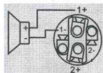
Speakon outputs-DA1004
