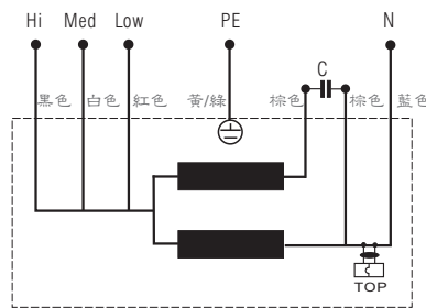
Single Phase Capacitor Motor Wiring Diagram
